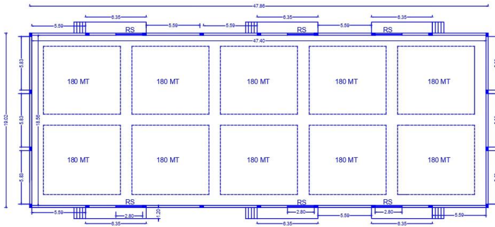
PLAN FOR 1800 MT WAREHOUSE SCALE 1:100
