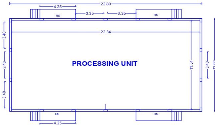
PLAN SCALE 1:100
