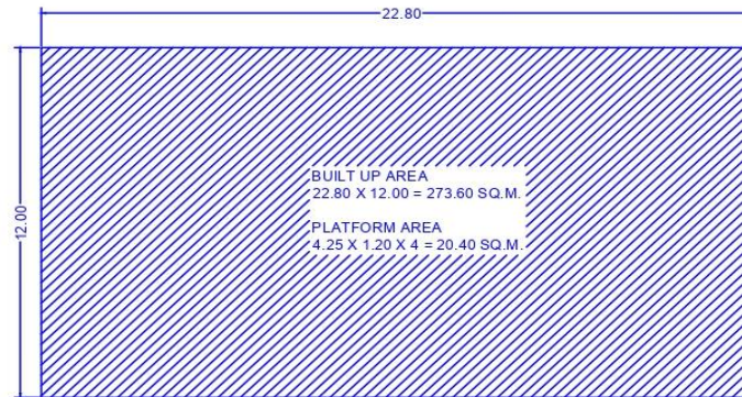
BUILT UP AREA SCALE 1: 100
